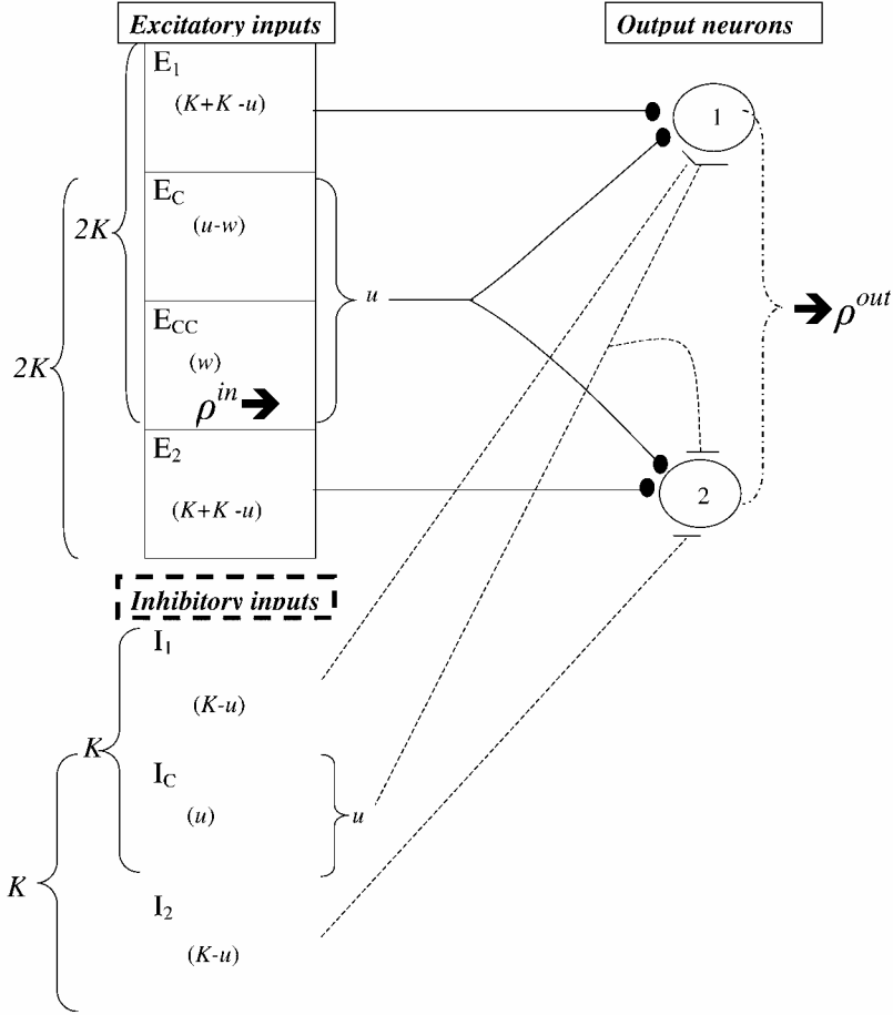
Figure 3: Two neurons of the same pool receive common input; the total input to each neuron is divided into five uncorrelated sub-fields: independent inhibitory and excitatory (E and I), common inhibitory and excitatory ( E_c and I_c ) and correlated common excitatory ( E_{cc} ) from the previous pool. Solid lines represent excitatory inputs, and dashed lines inhibitory inputs. Expressions in parentheses denote the number of synapses that establish each type of input. The total number of excitatory inputs is 2K , and the total number of inhibitory inputs that each neuron receives is K . Both neurons receive, on average, common input from u excitatory and u inhibitory neurons. The pairwise correlation assumed among inputs in E_{cc} , \rho^{in} , affects the correlation between the pair of output neurons, \rho^{out} .
