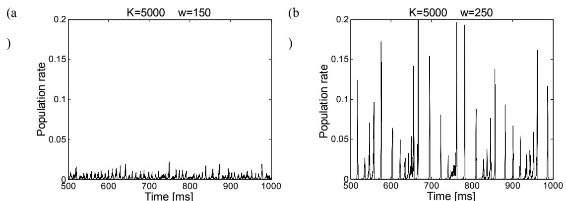
Figure 2: Population rate of a BN with embedded SFCs indicates a qualitative change in network behavior, as chain width increases. (a) With a chain of width w=150 , the network is in an AI state, characterized by low asynchronous population activity and very mild oscillations with
