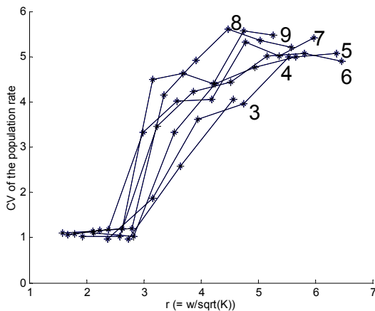
Figure 6: Scale invariance in the full network. The synchrony measure as a function of r , for different network sizes. Digits inside the figure denote the size of K in thousands. w range from
